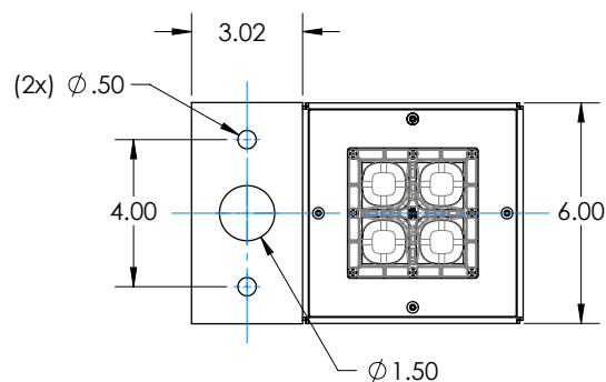
LYNXB- BASE TEMPLATE (2X) 3/8X18" L ANCHOR BOLT
